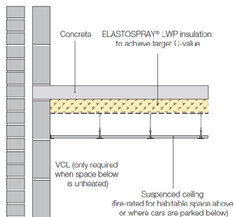
Diagram 1 - Internal soffit insulation
