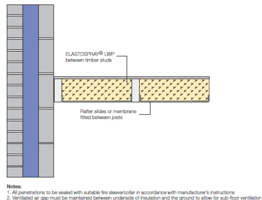
Diagram 2 - Insulation below suspended timber ground floor
